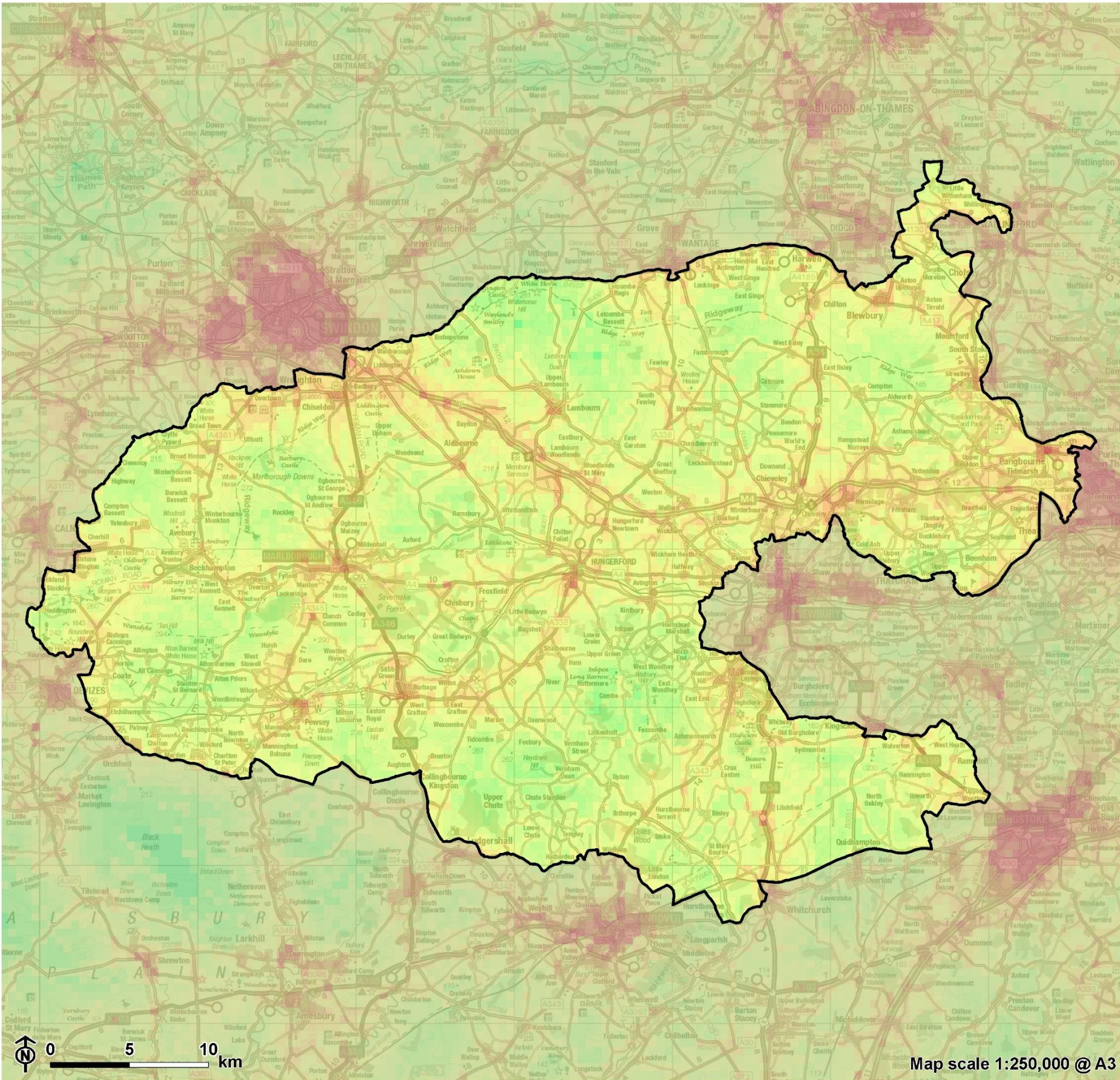
Figure 3.8: Tranquility
