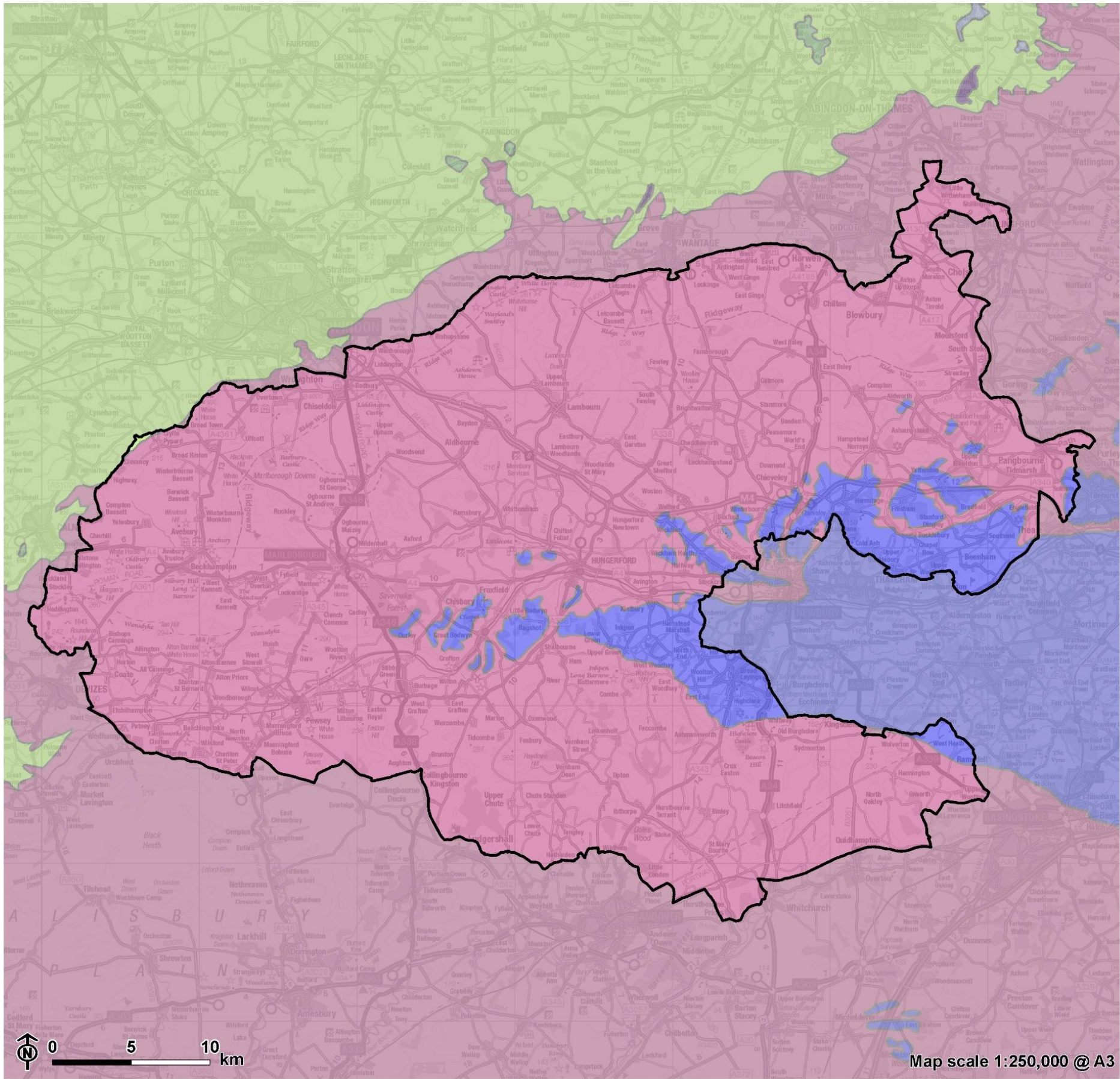
Figure 3.1: Bedrock Geology
